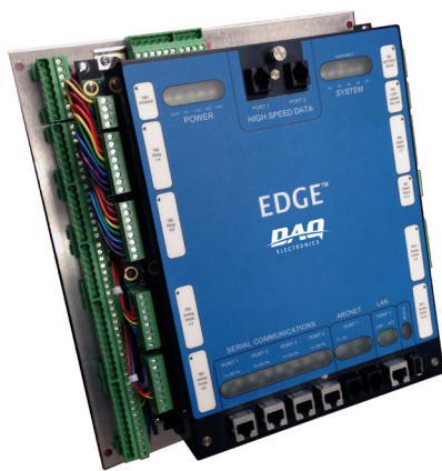
Shown mounted to an EDGE remote, the EDGE Conversion Panel provides an easy upgrade path for users of Polaris and Elara III units.
